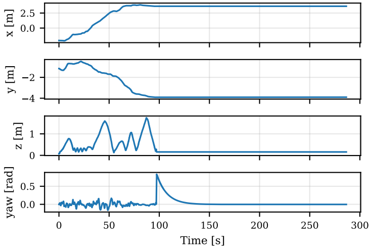
exp 9 - UAV 0 - Position
